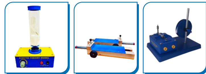
KINETIC THEORY
