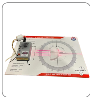
LASER OPTIC KIT
