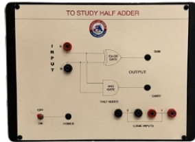
HALF ADDER
