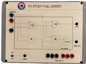
FULL ADDER
