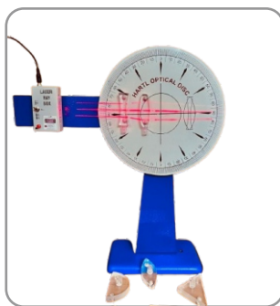
LASER HARTL OPTIC KIT
