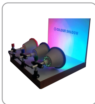
COLOURED SHADOW
