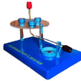
AMPERE'S LAW
