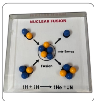
NUCLEAR FUSION
