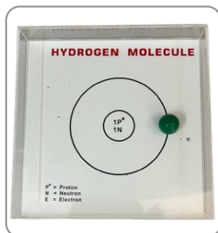
HYDROGEN MOLECULE
