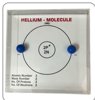
HELIUM MOLECULE
