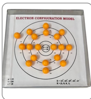
ELECTRON CONFIGURATION
