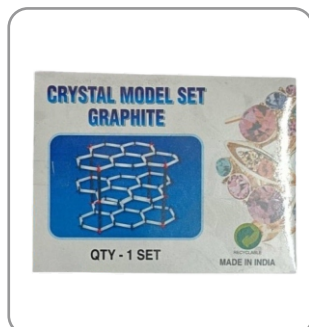
GRAPHITE MODEL
