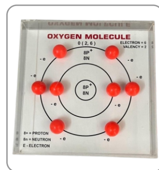
OXYGEN MOLECULE
