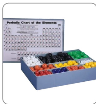
ATOMIC MODEL
